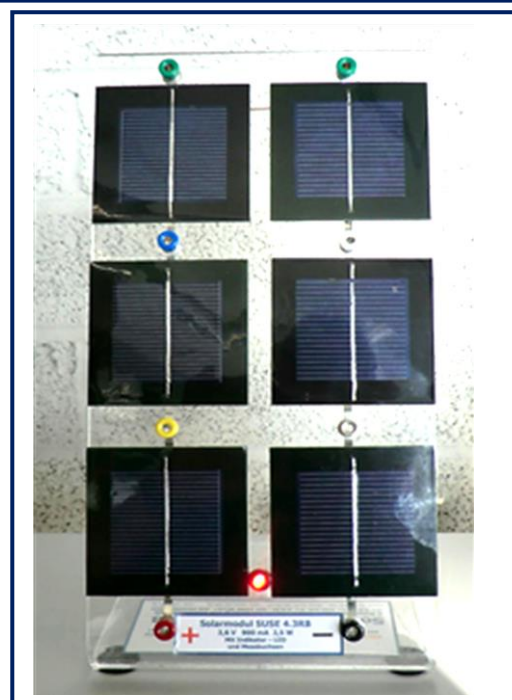
The solar module SUSE 4.3RB In the middle of the lower two solar cells the indicator LED is glowing. The total voltage is available at the lower black-red jack pair.
